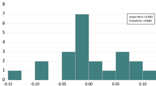
Figure 5. Results of normality test.
