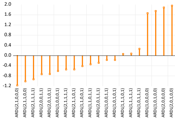
Figure 4. Alternative ARDL model selection based on the normalized Akaike Information Criterion (AIC).
