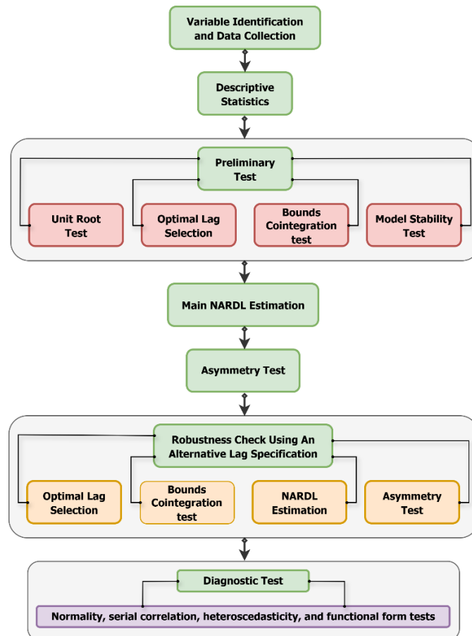
Figure 1. Study's empirical estimation procedures.
