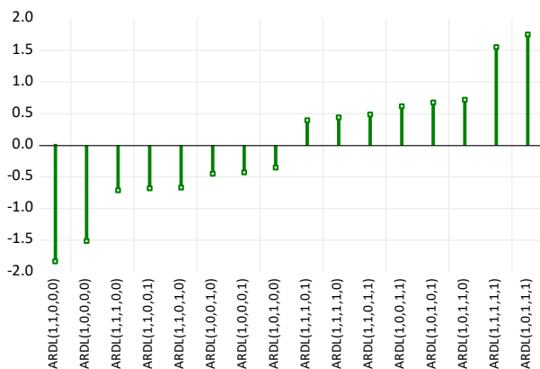
Figure 2. ARDL model selection based on the normalized Akaike Information Criterion (AIC).
