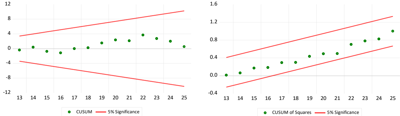
Figure 3. Results of CUSUM and CUSUMQ test.
